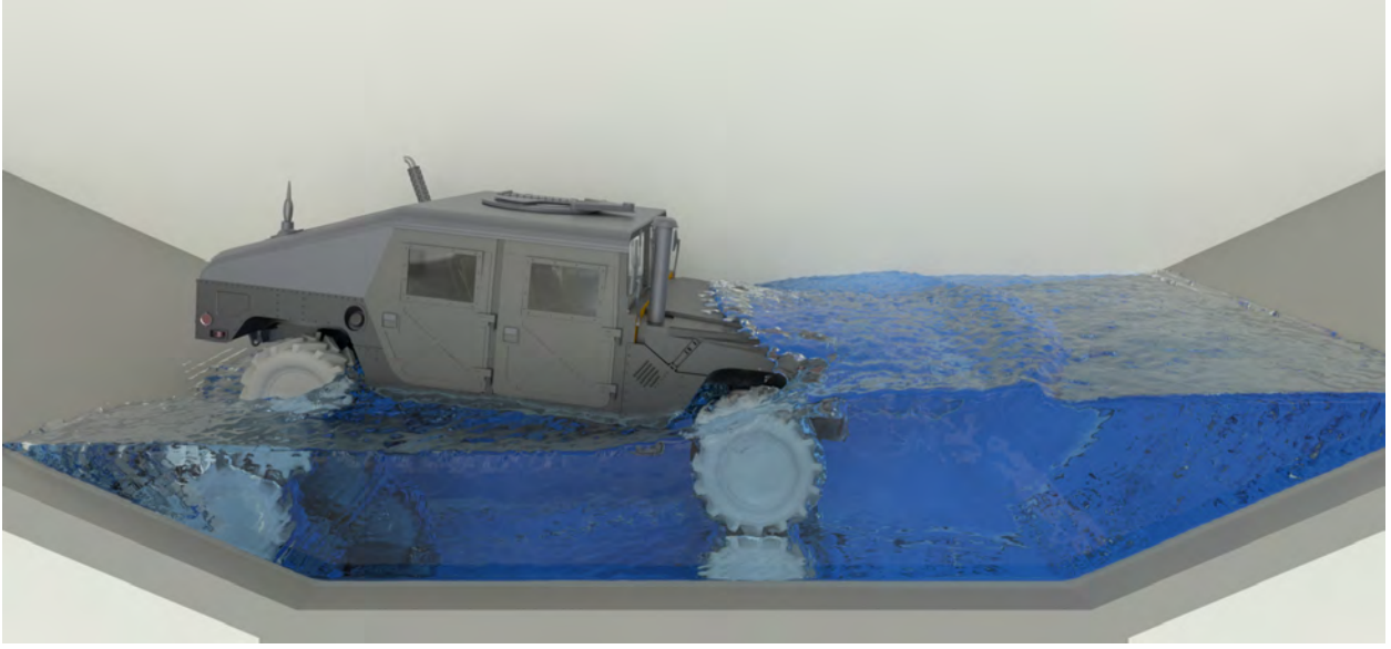
Fig. 7 Vehicle fording simulated using Chrono [34]. In this example, many features of Chrono are displayed, such as rigid body dynamics to simulate the interaction between the various components of the vehicle, flexible body dynamics to simulate the deformation of the tires, and SPH (smoothed-particle hydrodynamics) to simulate the interaction between the fluid and the vehicle body
