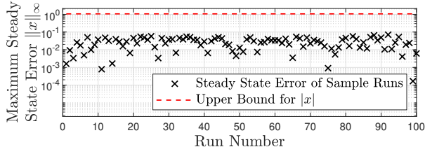
Fig. 2. Maximum steady-state error for the state x(\cdot) employing the 3/2 Matern-Sobolev kernel across 100 random simulations. The difference between this case and the Gaussian Kernel is negligible.
