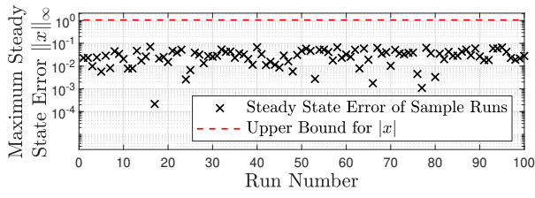
Fig. 1. Maximum steady-state error for the state x(\cdot) employing the Gaussian kernel across 100 random simulations. Conventional parametric approaches derive a different basis-dependent controller for each case. The upper bound is given by \sqrt{(1 + \mathcal{M}_{\infty}^2)f_{\infty}^2/4\beta c_1} .
